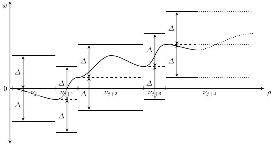
Fig. 4. Bounds on the cost of a request over time given by Lemma 6. We write \Delta = d'(n'W')^2 .
