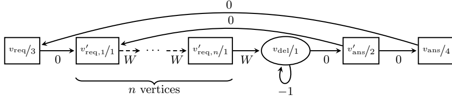
Fig. 5. A game of size \mathcal{O}(n) in which Player 0 only wins with strategies of size at least n2^n + 1 .
