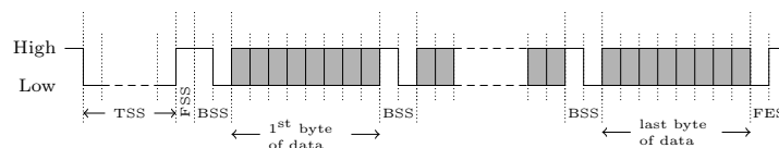
Fig. 2. Format of a message bit stream.
